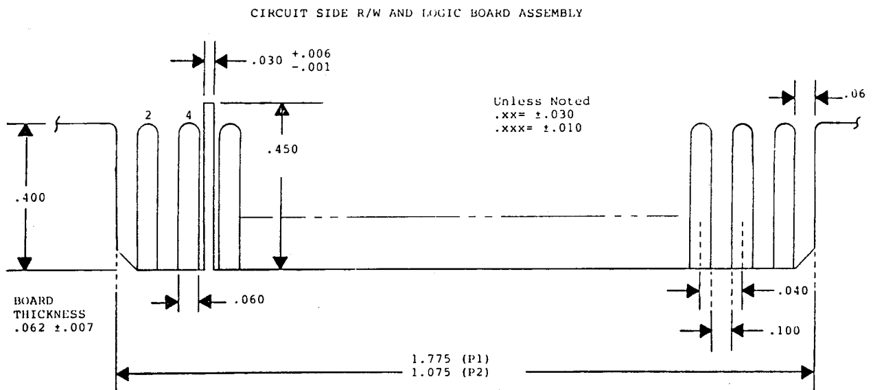
FIGURE 6-1 P1/P2 CONNECTOR
