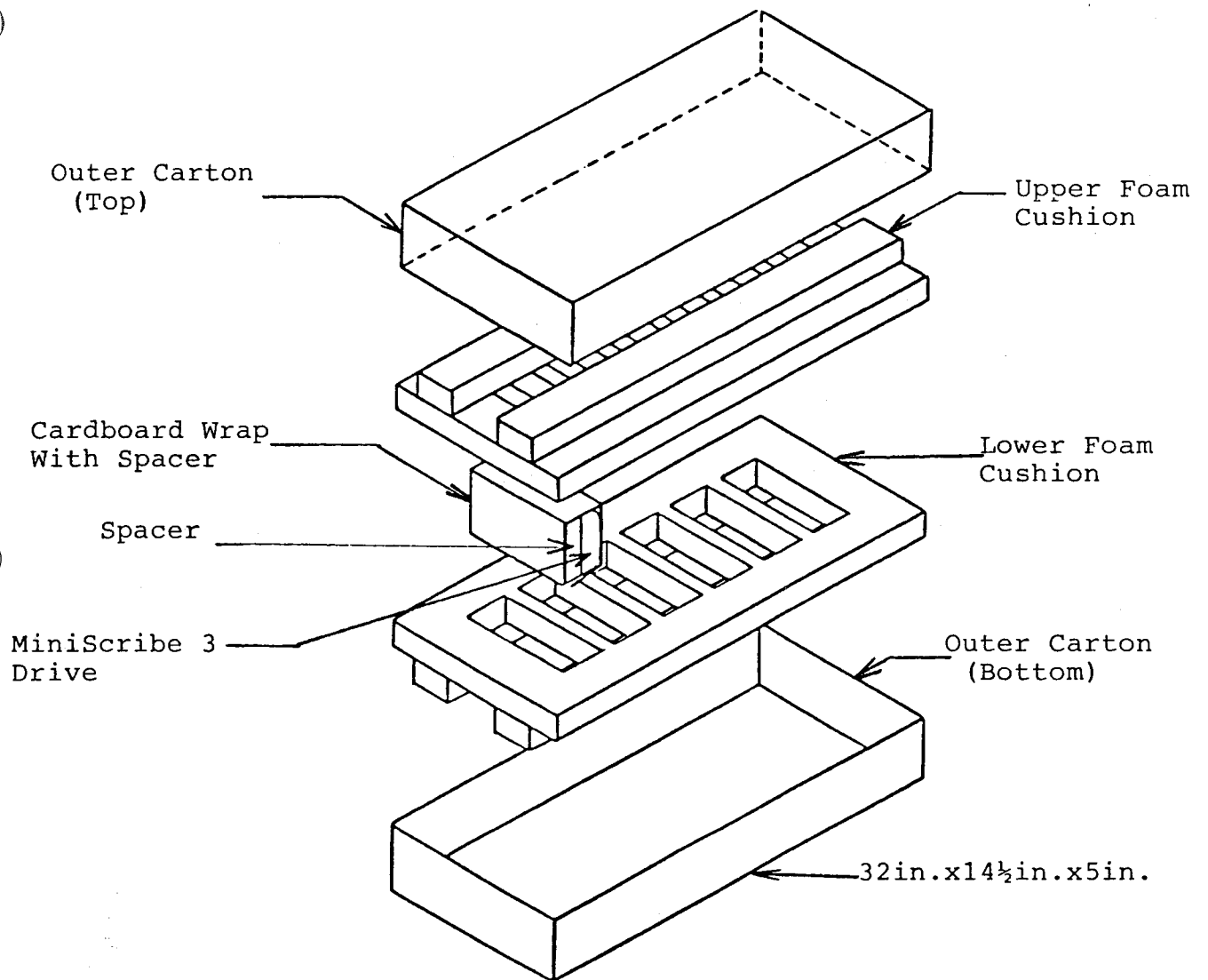
Figure 8-2 6 Pack Multipack Shipping Container
