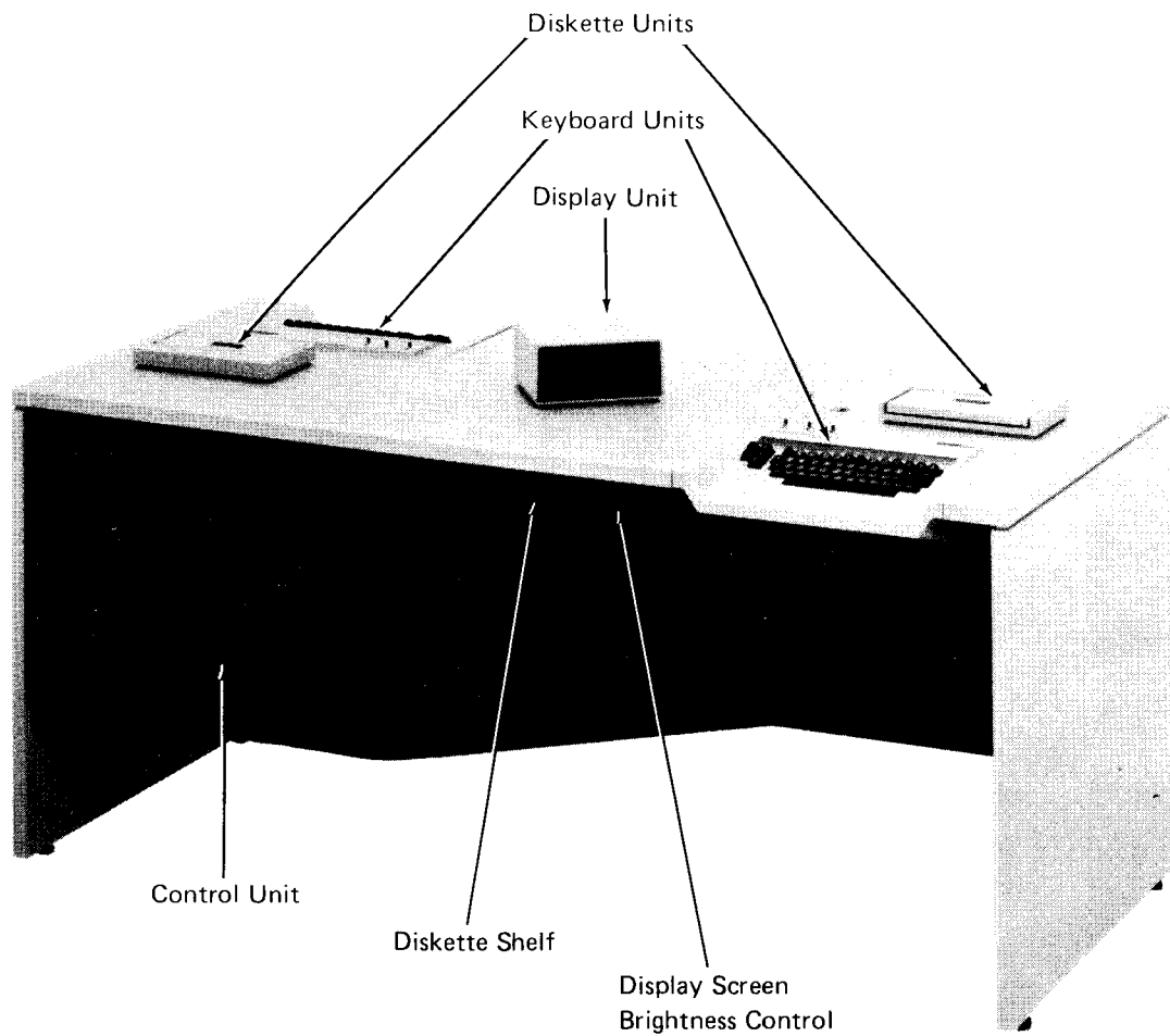
• Figure 1. IBM 3742 Dual Data Station
