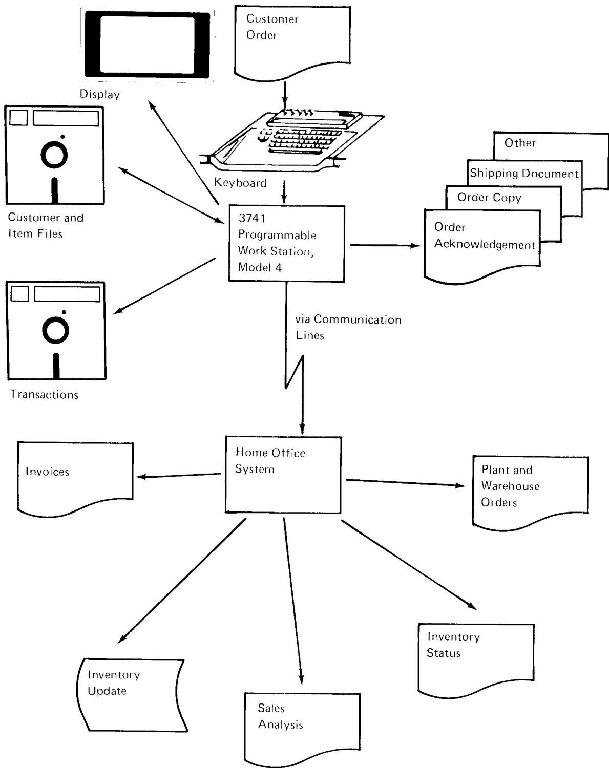
Figure 4. Warehouse Order Entry Data Flow
