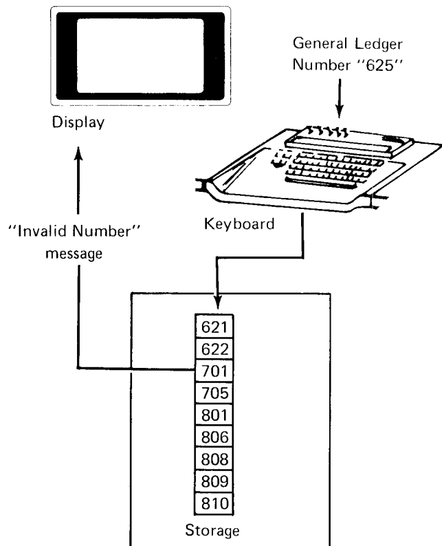
Figure 1. Table Search for Equal Entry
