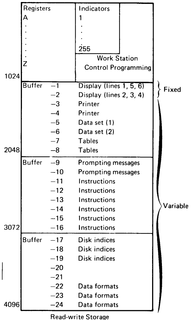
Figure 3. ACL Program Structure (4K)
