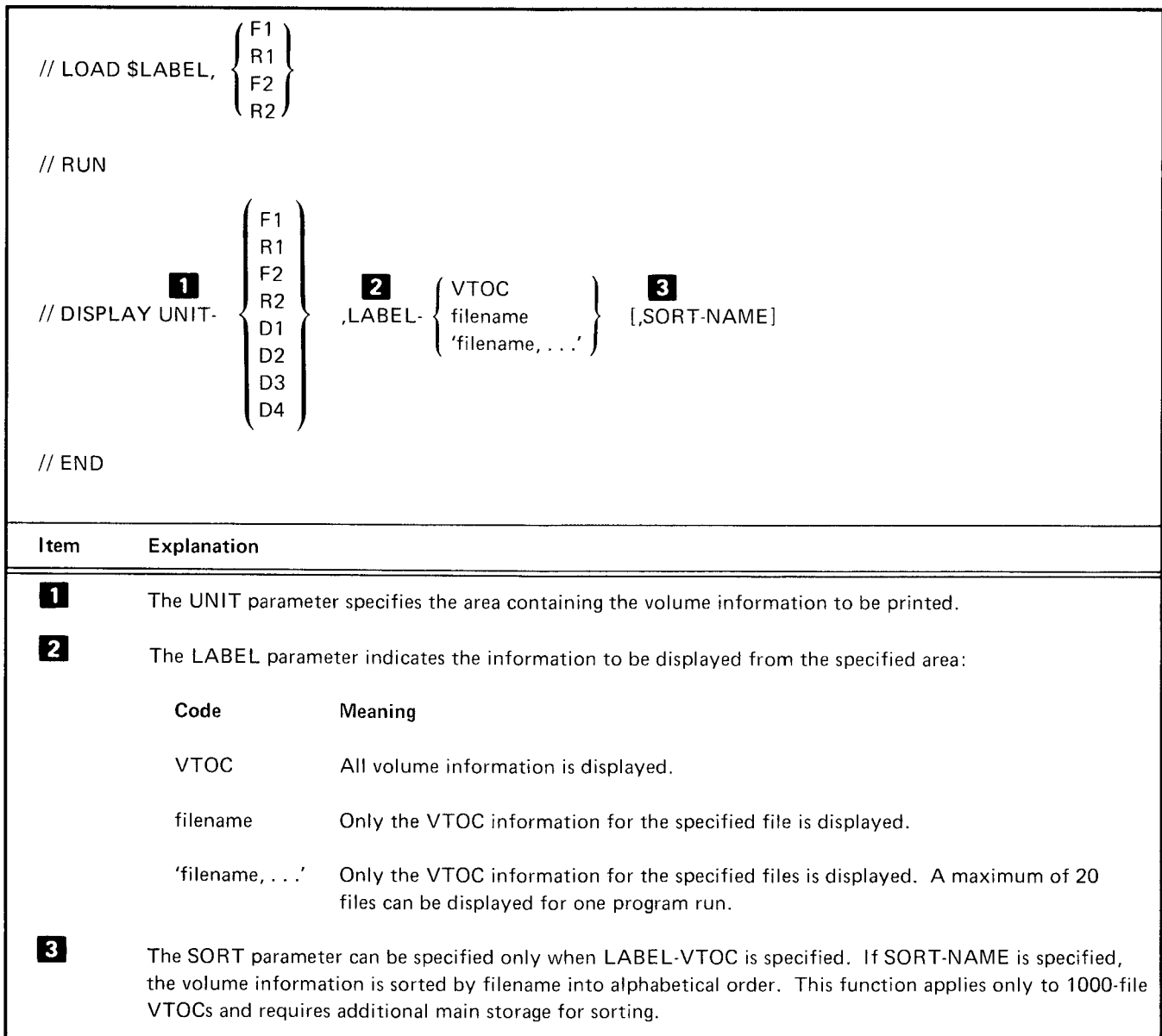
Figure 3-5. Control Statements Required for the File and Volume Label Display Program
