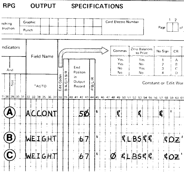
Figure 3-20. Edit Words
