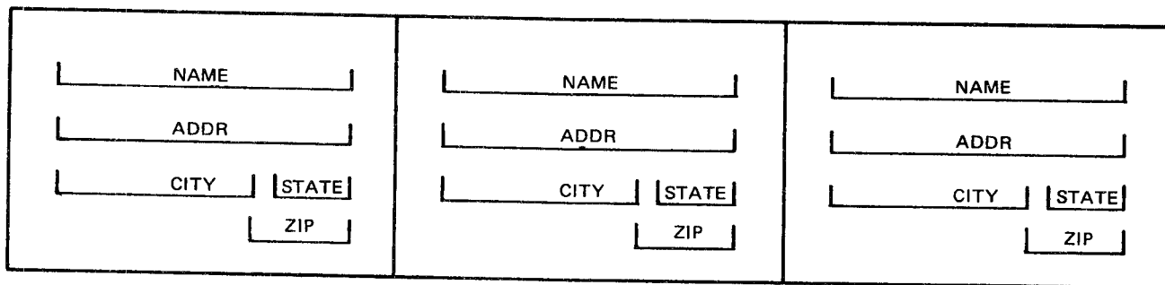
Figure 3-30. Mailing Labels
