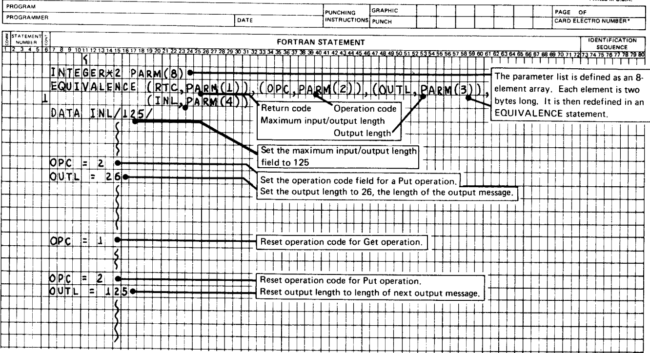
Figure 5-3. Setting Elements in the Parameter List Array
