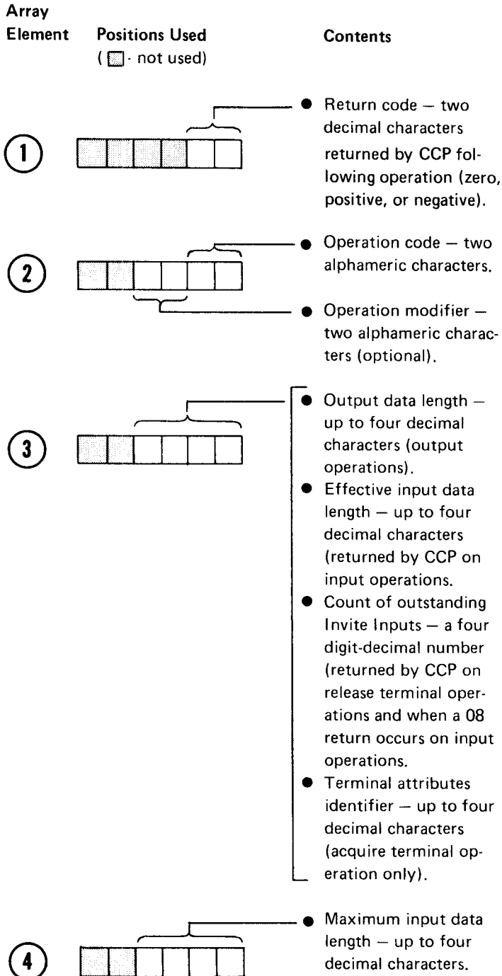
Figure 6-12. RPG II Parameter Array for EXIT/RLABL
