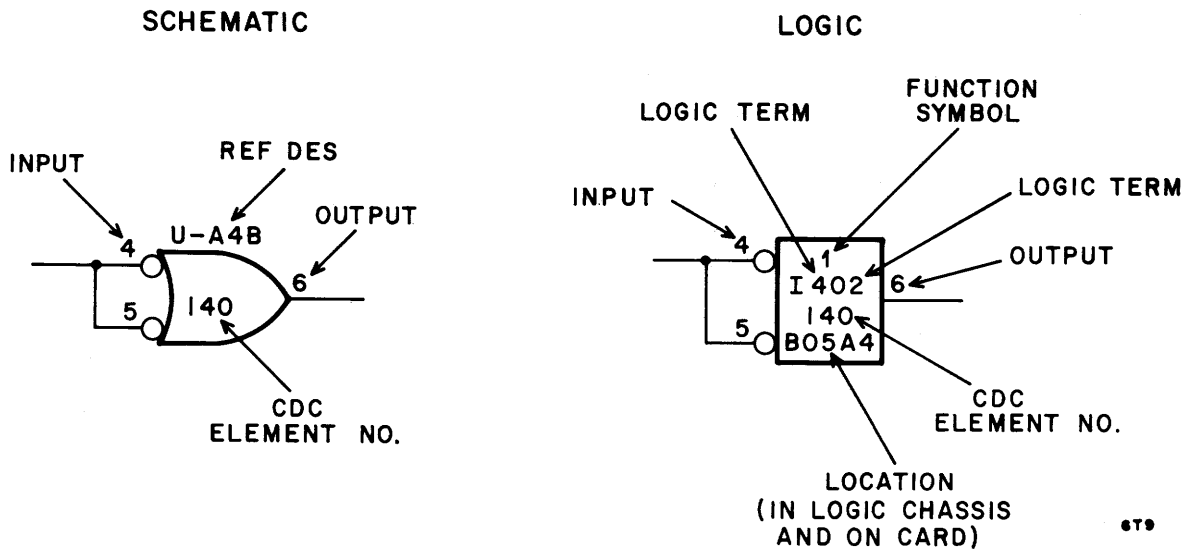
Figure 7-4. Integrated Circuit
