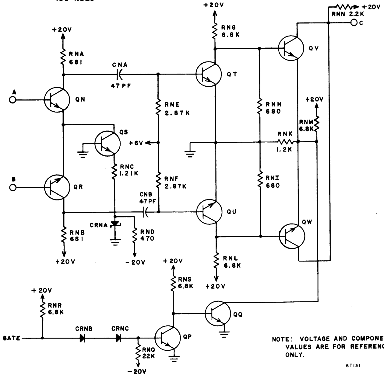
Figure 7-68. Gated Single Shot - XAC
