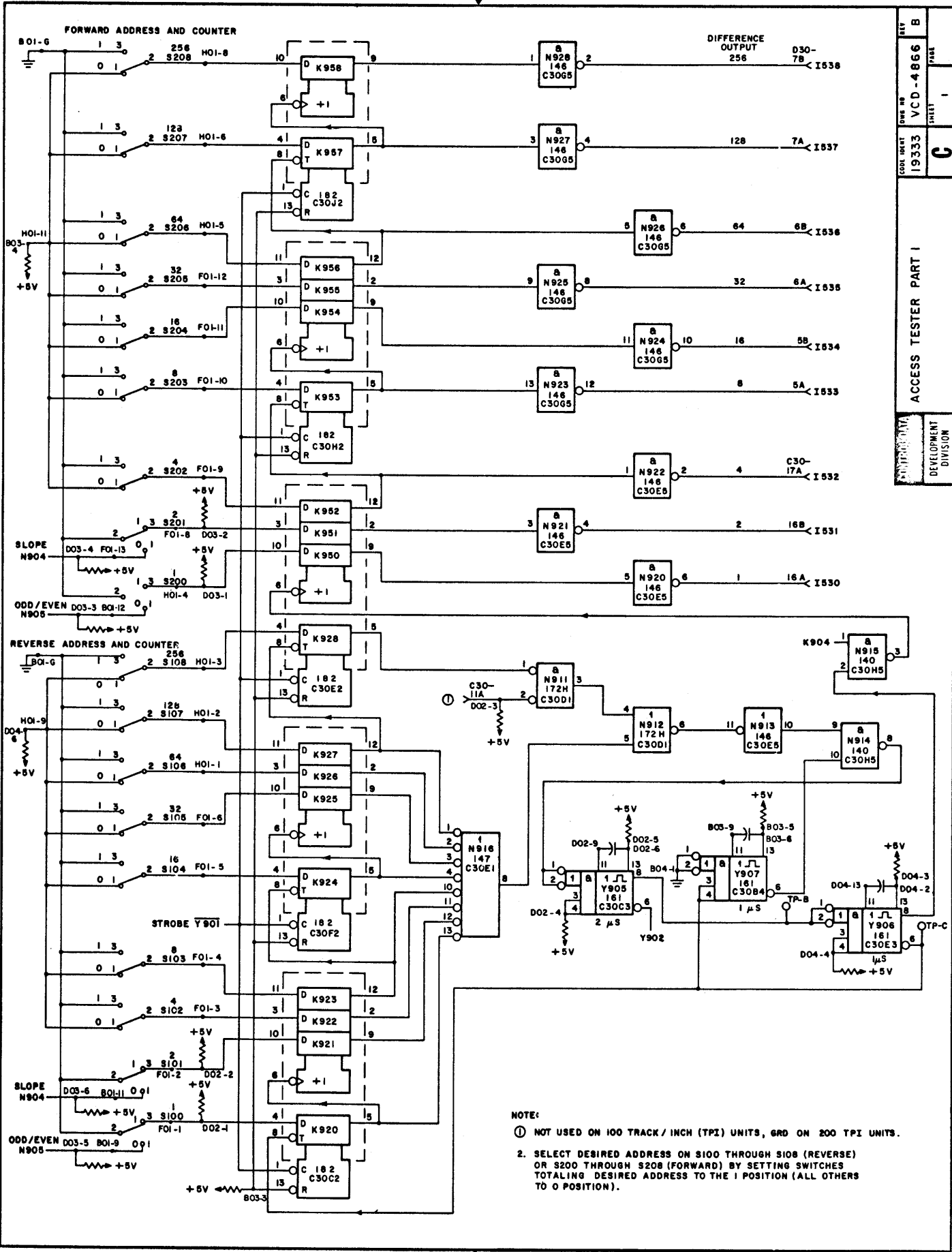
Figure 7-71. Access Tester Card Logic - (Sheet 1 of 2)
