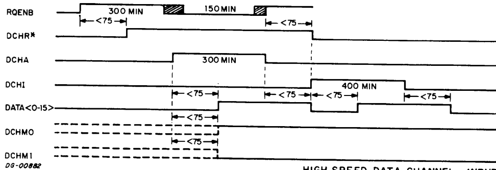
HIGH SPEED DATA CHANNEL - INPUT
