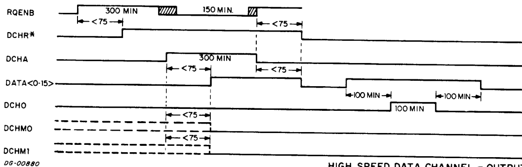
HIGH SPEED DATA CHANNEL - OUTPUT
