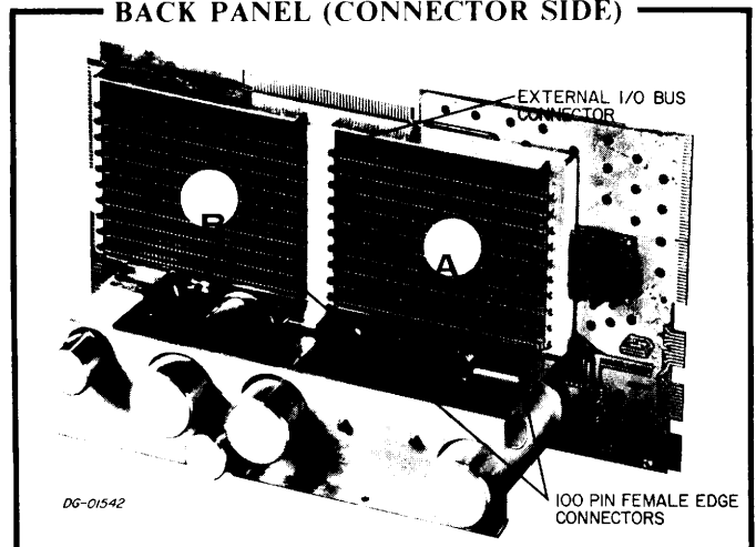
BACK PANEL (CONNECTOR SIDE)
