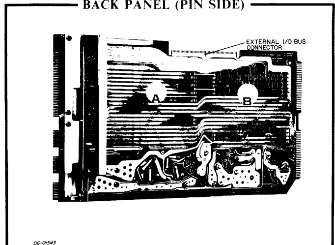
BACK PANEL (PIN SIDE)
