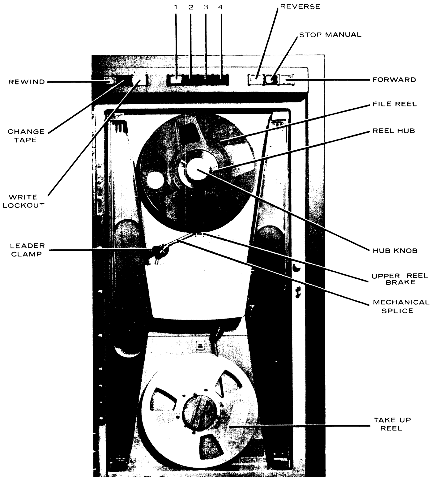
Figure 4-9. 1607 Tape Unit
