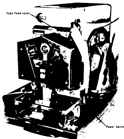
Figure 4-6. Paper Tape Punch
