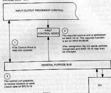
Figure 11.11 Exchange Cycle CW1
