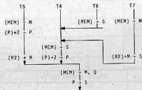
Figure 8.2 Microprogram Addressing Routine
