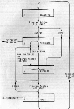
Figure 11.2 Four states of standard control unit
