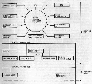
Figure 1.1 System Main Components
