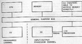
Figure 11.1 Units concerned with transfers
