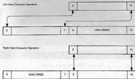
Figure 4.1 Operation of memory in character mode
