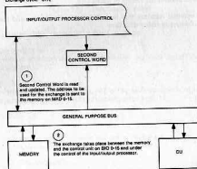
Figure 11.12 Exchange Cycle CW2
