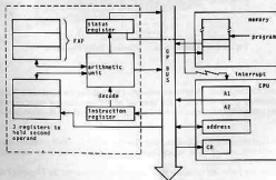
Figure 6.2 Floating Point Processor
