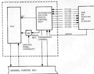
Figure 14.1 Integrated serial control unit
