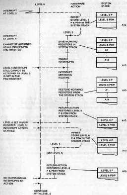
Figure 10.1 Diagram of interrupt sequence
