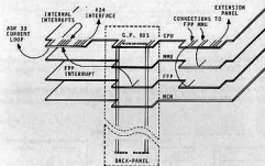
Figure 6.1 Connection of Floating Point Processor
