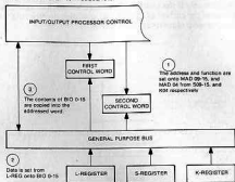
Figure 11.9 WER Instruction Flow
