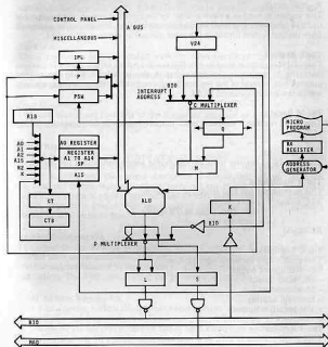
Figure 2.2 Data flow in Data Handling Unit
