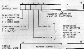
Figure 11.6 I/O Processor Control Words
