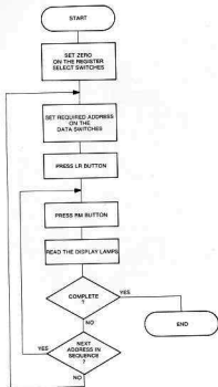
Figure 13.4 Displaying Memory Contents
