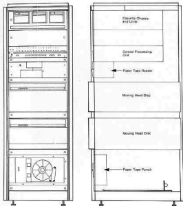
Figure 16.2 Example of Equipment Mounted in a Cabinet
