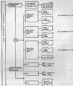
Figure 1.2 Survey of peripherals and their control units
