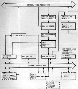
Figure 2.1 General structure of CPU
