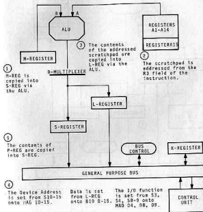
Figure 11.4 OTR/CIO Instructions Flow
