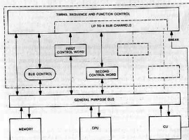
Figure 11.7 I/O Processor within the system
