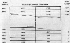
Figure 4.2 Layout of words and characters in memory.
