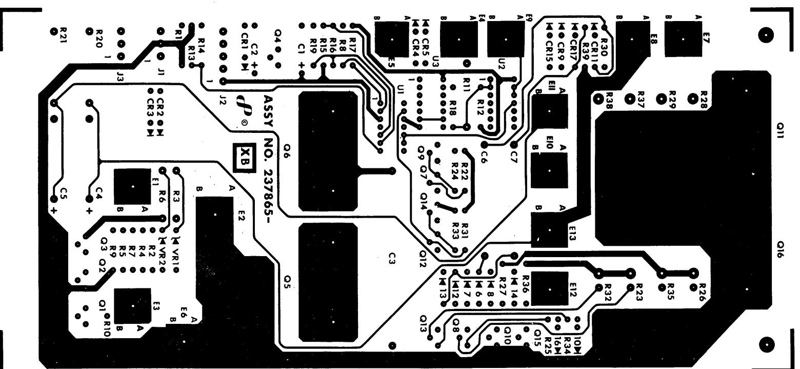
Figure 9-21 Hammer Supply Circuit Card Assembly
