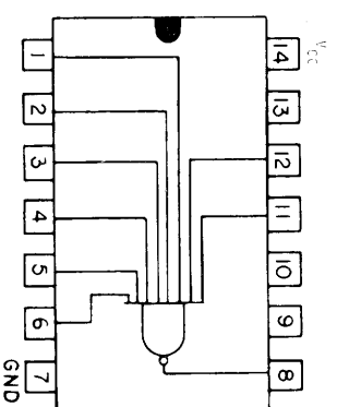
SINGLE 8 INPUT NAND GATE 800021-001 DPC 7430 800021-002 (HERMETICALLY SEALED)
