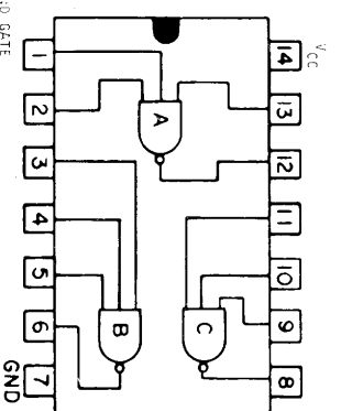
TRIPLE 3-INPUT NAND GATE 800023-001 DPC 7410 800023-002 (HERMETICALLY SEALED)
