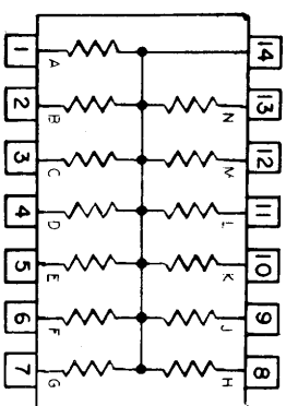
RESISTOR, NETWORK PULL-UP, 13 RESISTORS 801006-
