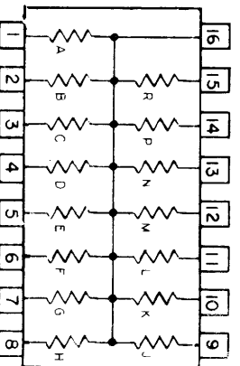
RESISTOR, NETWORK PULL-UP, 15 RESISTORS 801008-
