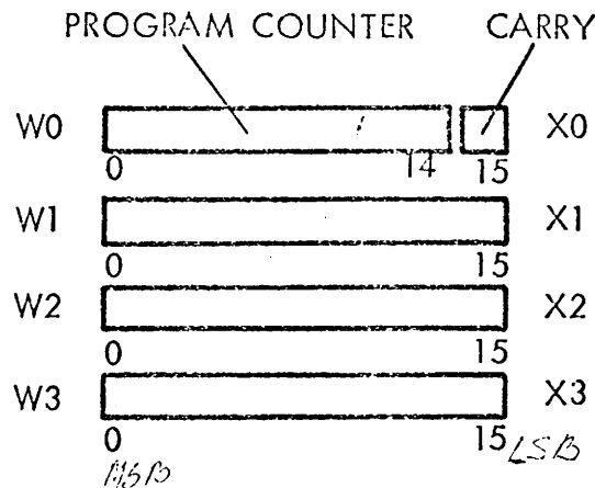
Figure 2.1.1. A Set of Working Registers
