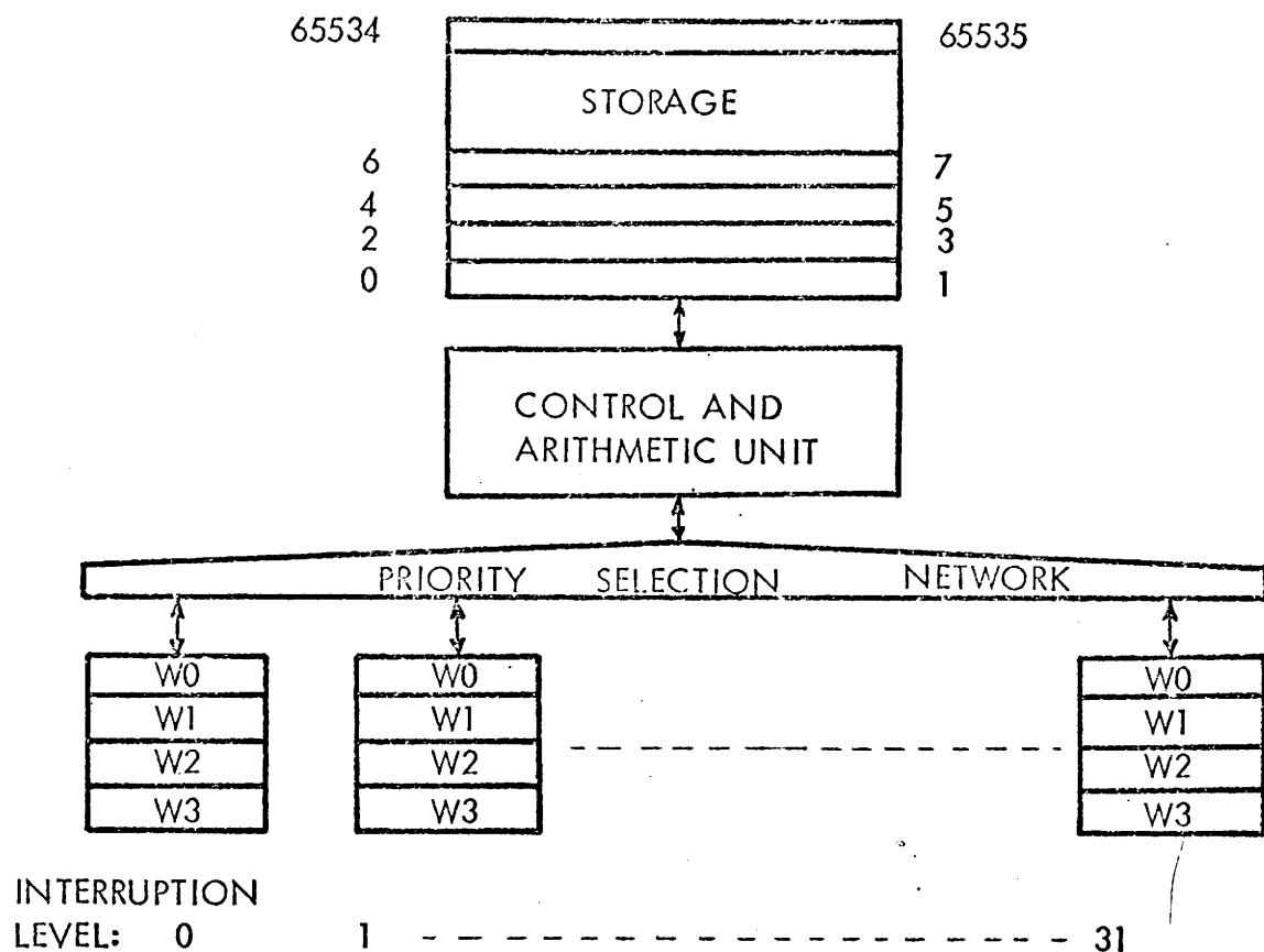
Figure 2.6.1. 3500 Block Diagram
